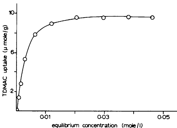
Fig. 1. Sorption isotherm of TDMAC by PVC from toluene solution at 20°C.
